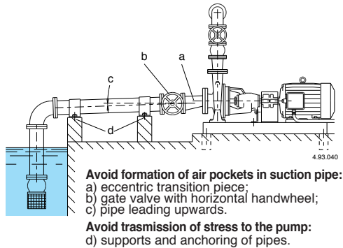
Fig. 4 Connection of pipes.
